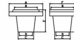
BT50
