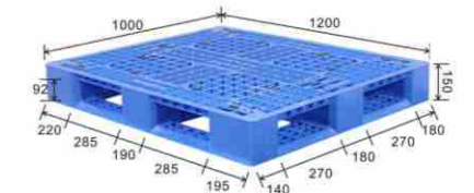
Plastic pallet 塑料托盘
